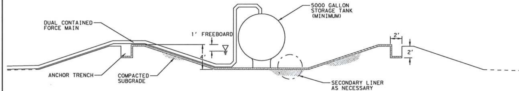
TYPICAL CONTAMINATED WATER STORAGE TANK AND BERM DETAILS N. T. S.
